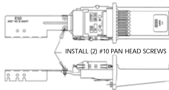
MOUNT WASHER EXTENSION #20697 TO COIN SLIDE
