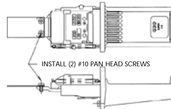
MOUNT DRYER EXTENSION #21420 TO COIN SLIDE
